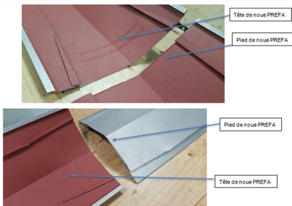
Figure 15 - Noue PREFA (pente minimum 33 %)
