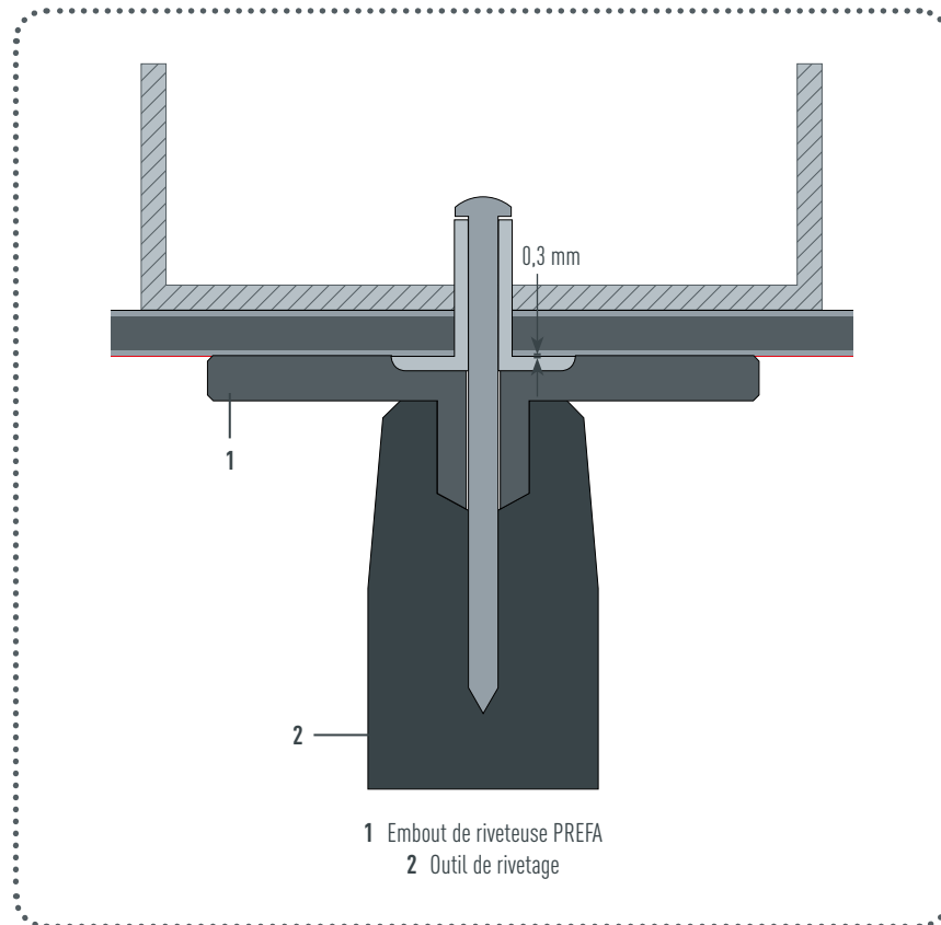
Figure 2 - Rivets de balcon PREFA
